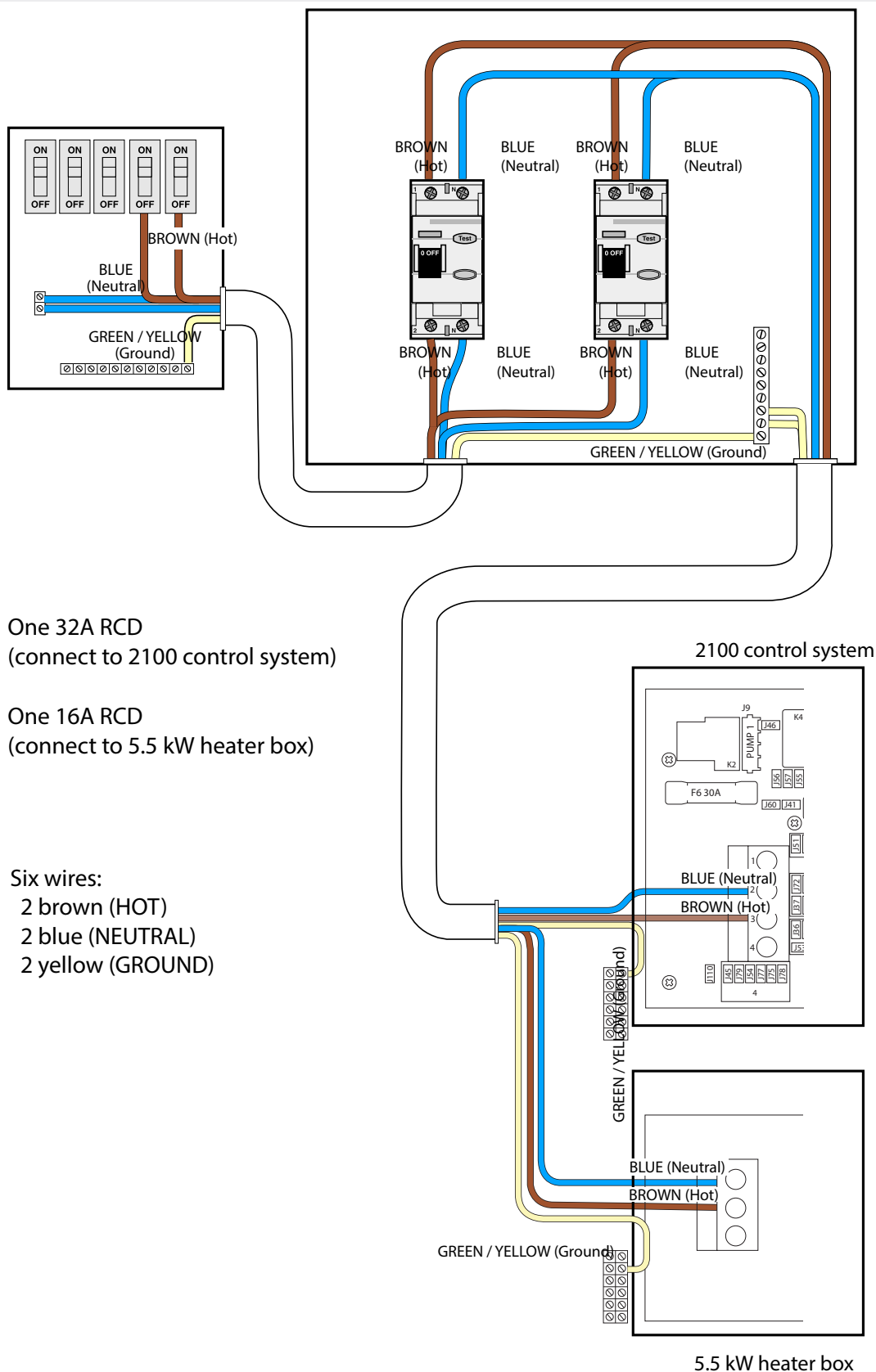
Diagram 4 230 Volts 50 Hz
