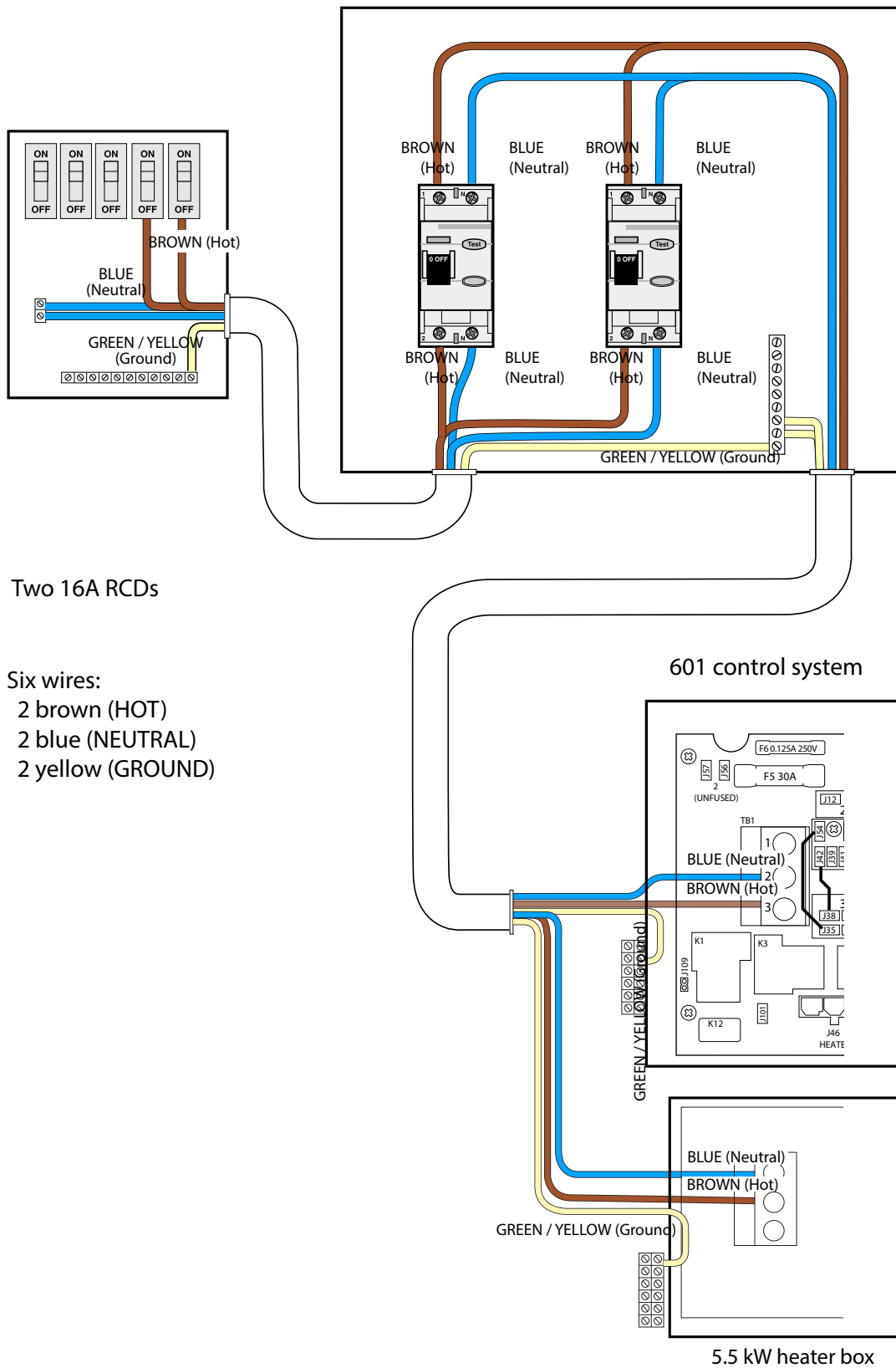
Diagram 3 230 Volts 50 Hz
